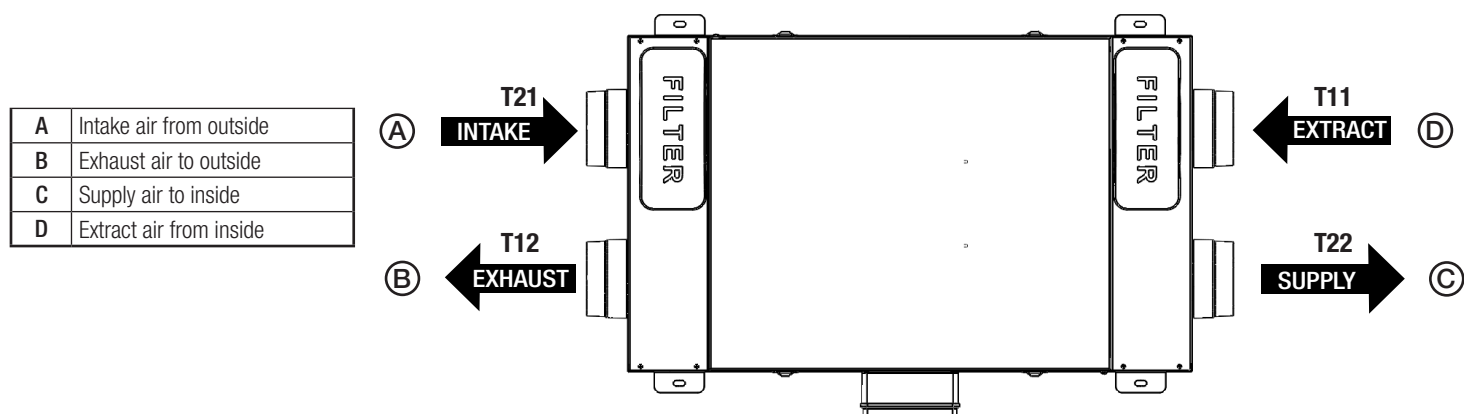
Fig. 7.a Temperature probes
