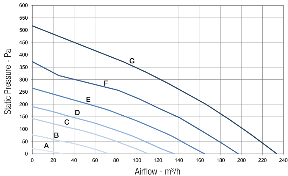
Fig. 6.a Performance curve
